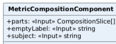
Figura 118: Classe: MetricCompositionComponent
