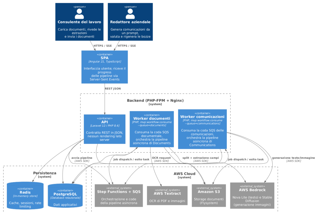
Figura 2: Container Diagram
